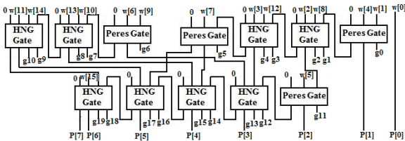
Figure 3: Reversible multiplier Product generation stage
