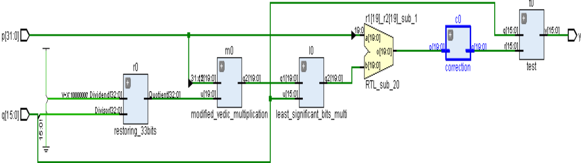
Figure 8: RTL schematics of the barett reduction algorithms
