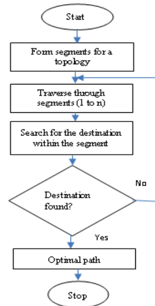
Fig. 4. Flowchart for Beehive algorithm
