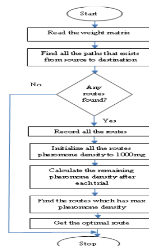
Fig. 2. Flowchart of ACO algorithm
