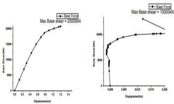
Figure: 9 X-YDIRECTION
