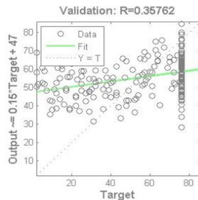
Figure 10. Target validation of the sample.
