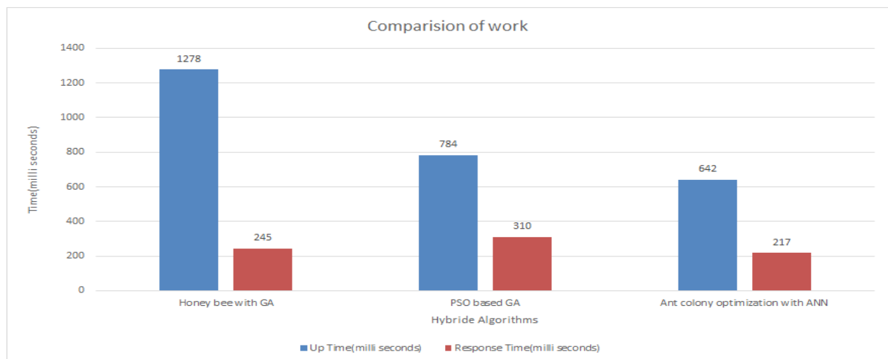
The hybrid ACO-ANN is compared with the existing technique, honeybee with GA and PSO with GA.
