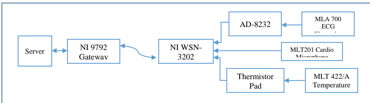
Figure 2- Connection Scheme
