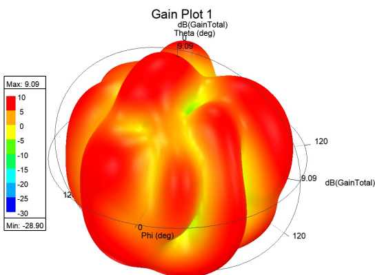
Fig. 12. Gain (design2)
