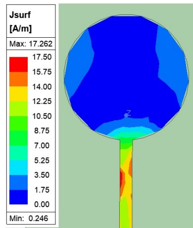
Fig. 20. surface current3
