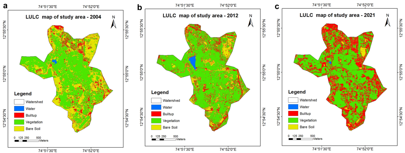
Fig. 7 Land cover details of the study area in the year of a 2004 b 2012 c 2021
