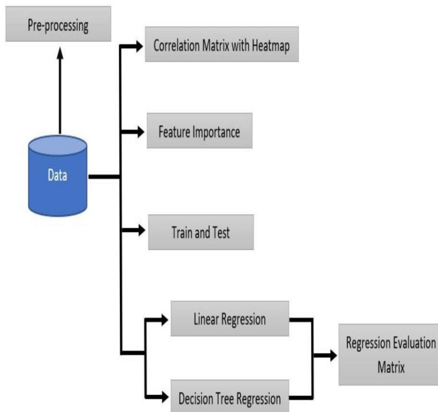
Figure 2.2 Data flow Diagram
