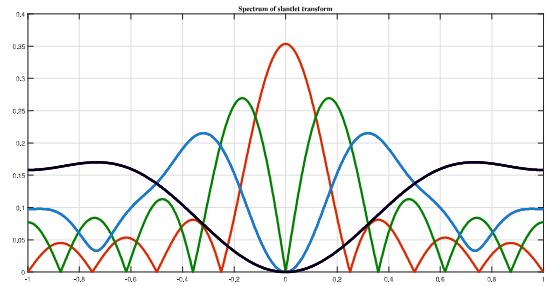
Fig. 7. Spectrum of Slantlet filter coefficients
