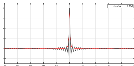
Fig. 12. Comparison of auto-correlation between LFM and slantlet radar waveform
