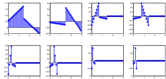
Fig. 8. The waveforms of the individual Slantlet Filter coefficients
