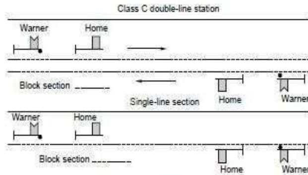
Fig. 26.3 C class station
