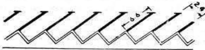
ANGLE PARKING
