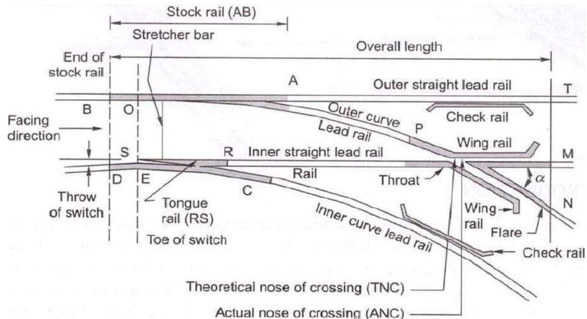
Fig. (a) Constituents of a turnout
