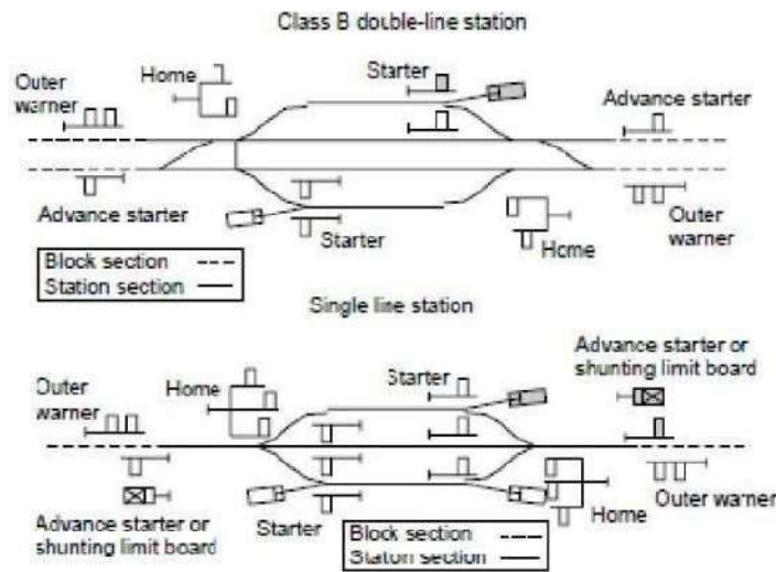
Fig. 26.2 B class station
