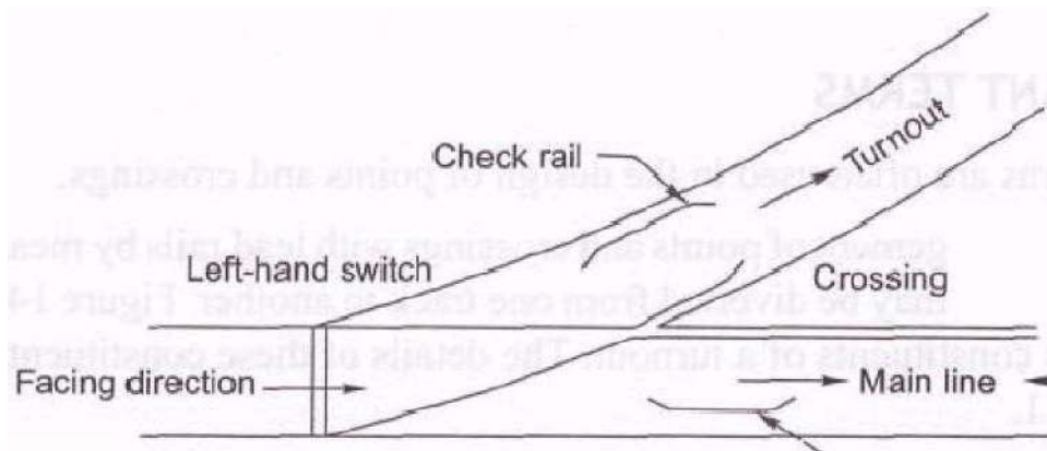
Fig. (b) Left-hand turnout
