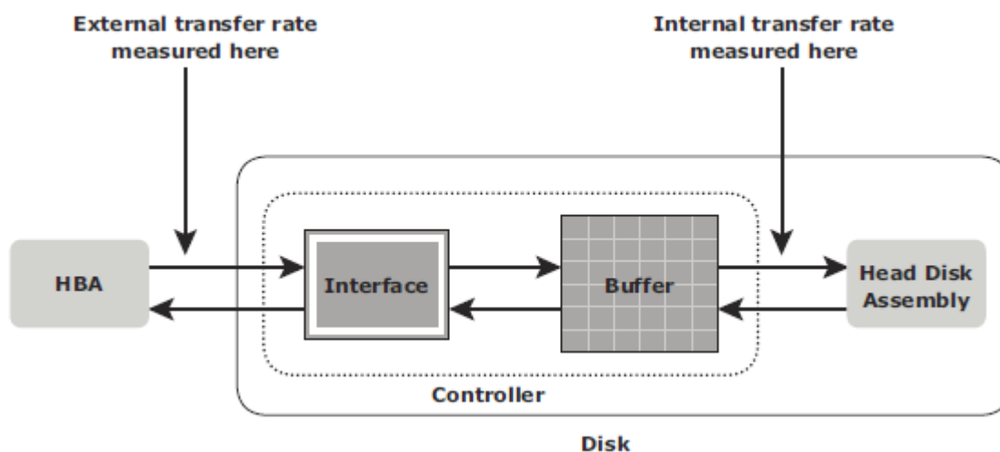
Fig 1.17: Data transfer rate
