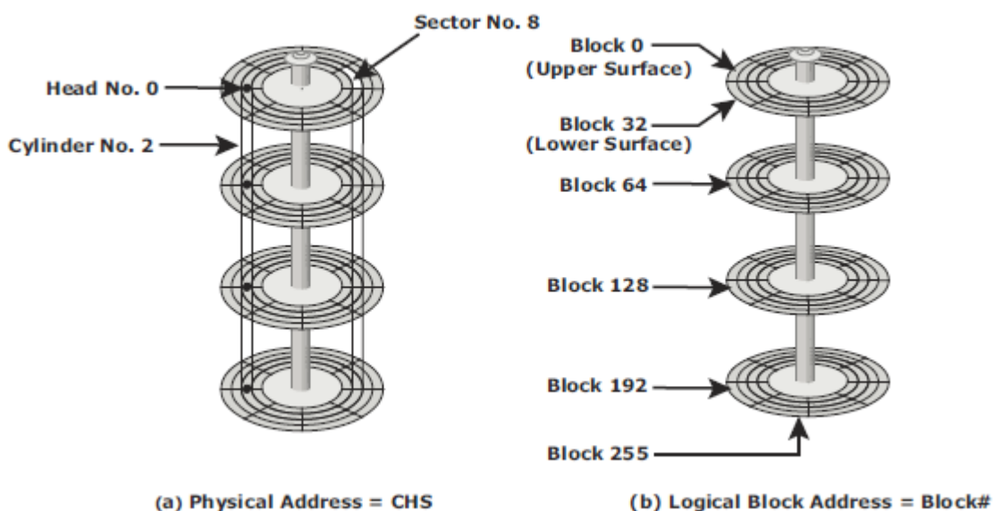
Fig 1.16: Physical address and logical block address
