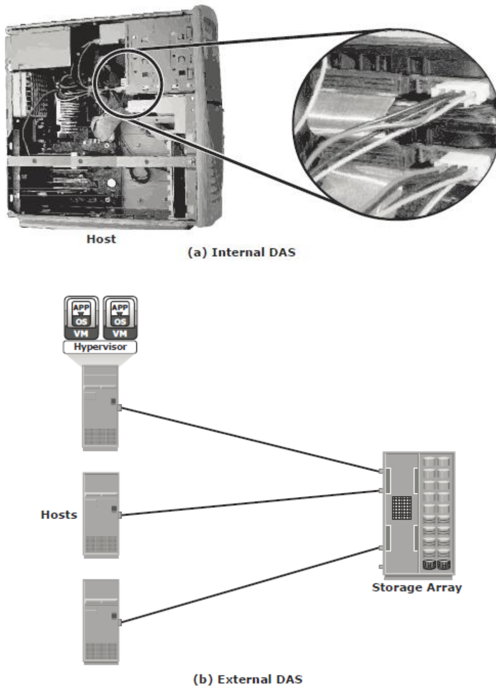
Fig 1.21: Internal and external DAS architecture
