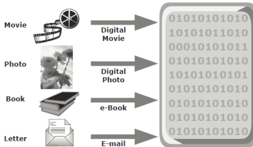
Fig 1.1: Digital data
