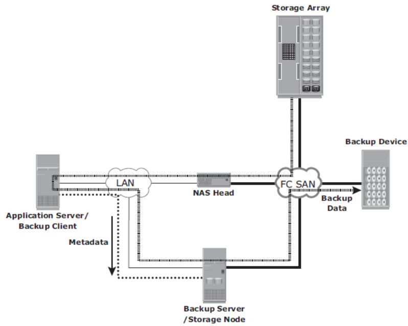
Figure 10-11: Server-based backup in a NAS environment
