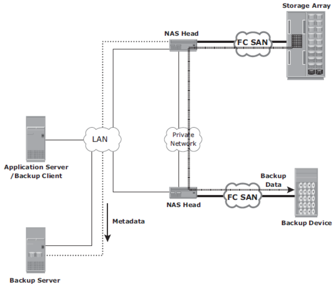
Figure 10-14: NDMP 3-way in a NAS environment
