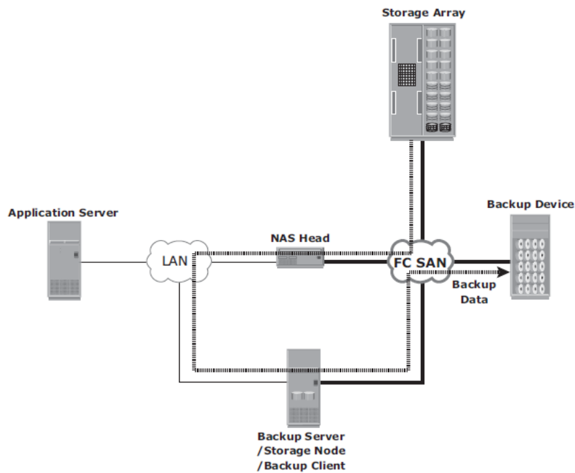
Figure 10-12: Serverless backup in a NAS environment
