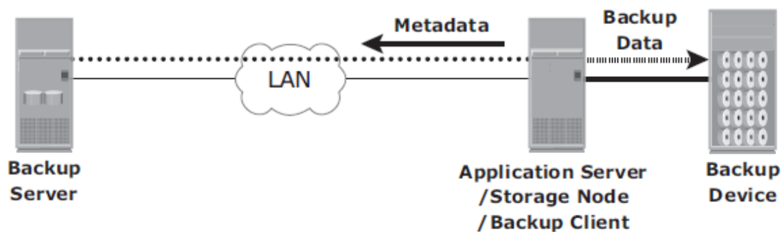
Figure 10-7: Direct-attached backup topology
