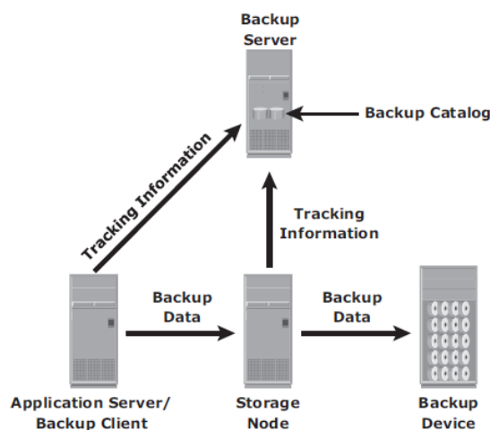
Figure 10-4: Backup architecture
