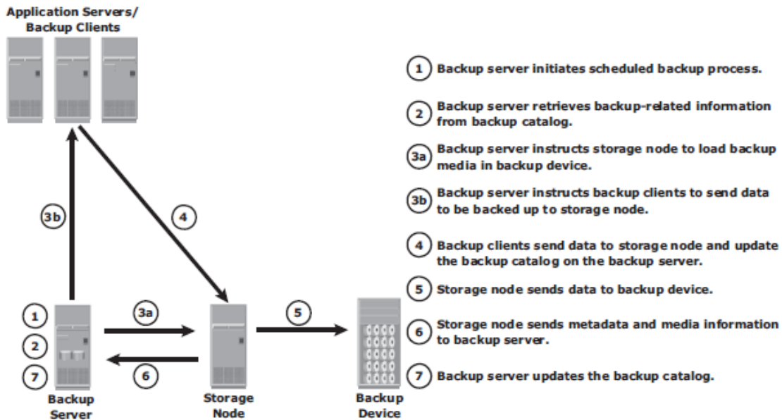
Figure 10-5: Backup operation
