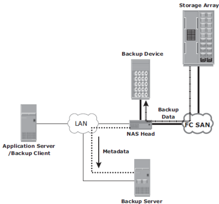
Figure 10-13: NDMP 2-way in a NAS environment
