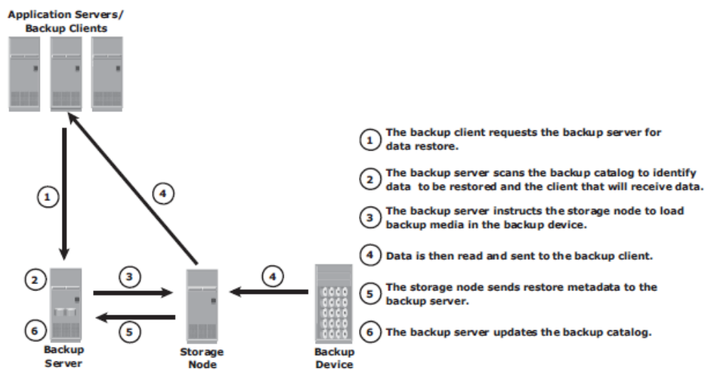
Figure 10-6: Restore operation
